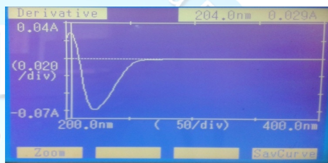
Fig. 4: first order derivative spectrum of Saxagliptin
