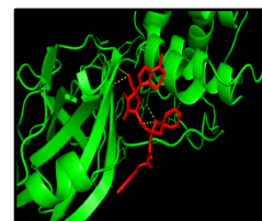
Interaction Analysis
