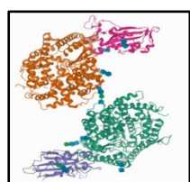
Protein Preparation
