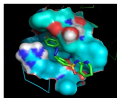
Docking/Screening
