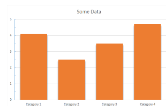
Energy calculations
