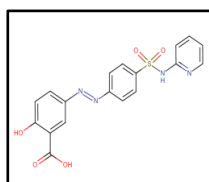
ligand Preparation
