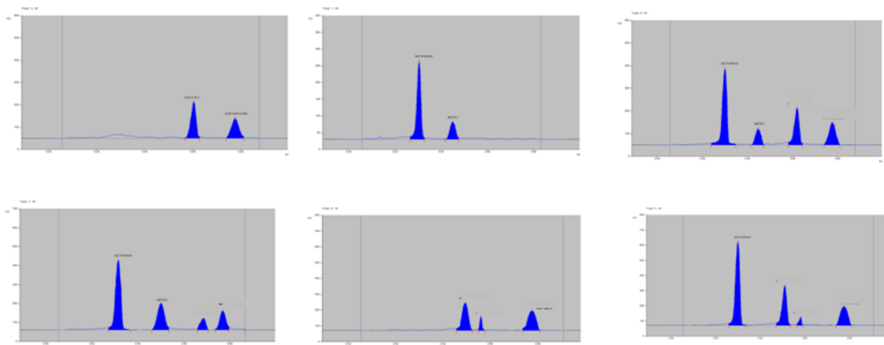
Fig 2. Densitogram of forced degradation of mixture of Empagliflozin and Metformin under various Conditions
