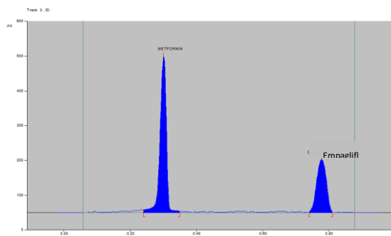
Fig 1. Densitogram of mixture of Empagliflozin and Metformin standard
